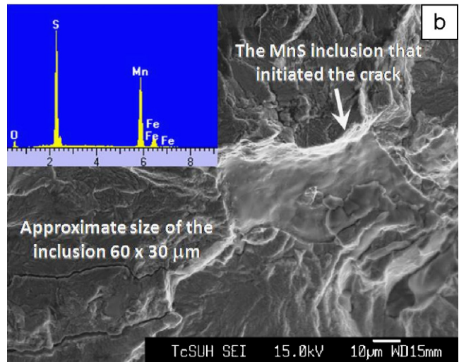
Fig. 5. Crack surface of a Class C wheel sample tested under uniaxial fatigue (a) fracture and (b) MnS inclusion that initiated the failure.
